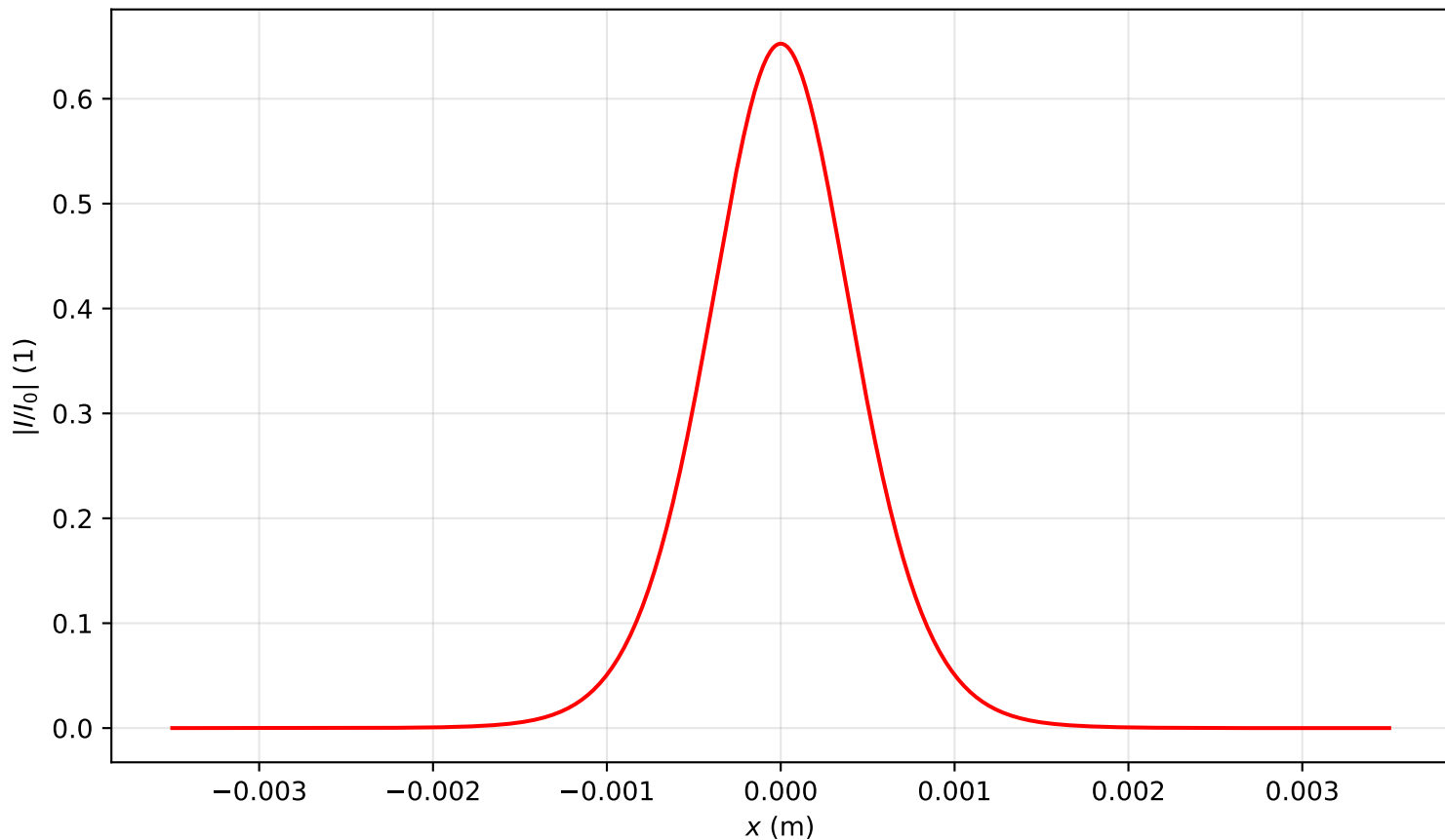
Intensity profile I(x, y = 0, z = 2.627)/I_0 , \text{Pin}=0.5\text{Pcr} , artificial time
